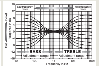
Tone control characteristics
