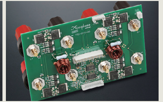
Protection circuitry
